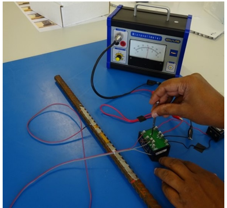
Figure 3. Bridge Balancing with Adjustment Potentiometer
