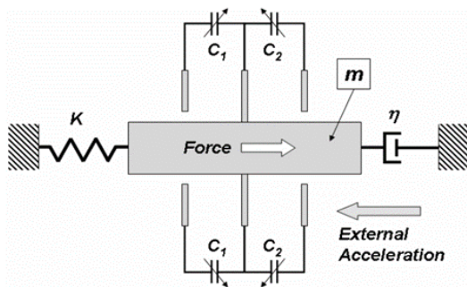
Figure 5. Schematic mechanical system of a capacitive accelerometer
