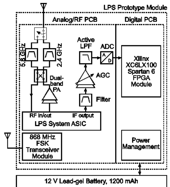
Figure 2. LPS prototype module block diagram
